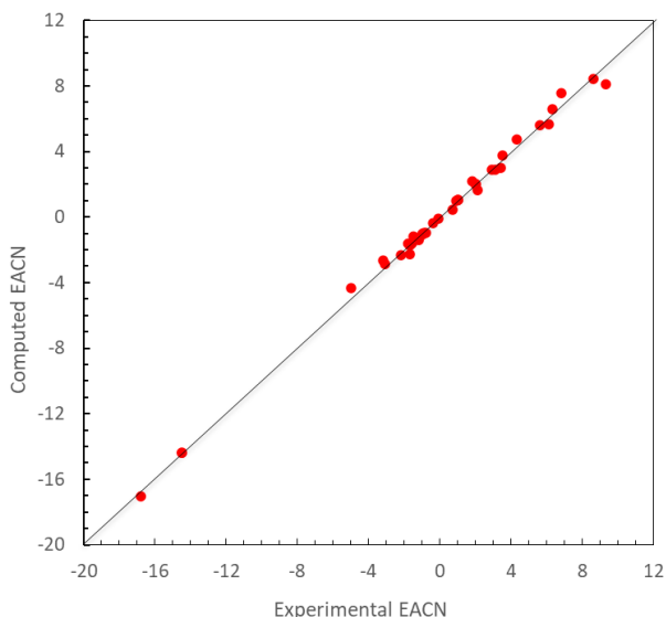
Fig. 2. Comparison of computed and experimental values of EACN for 58 fragrances and perfumery raw materials
