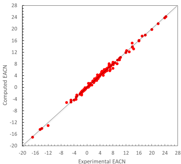
Fig. 1. Comparison of computed and experimental EACN values for 141 hydrophobic compounds
